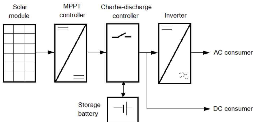
Figure 1. Block diagram of an autonomous solar power plant
