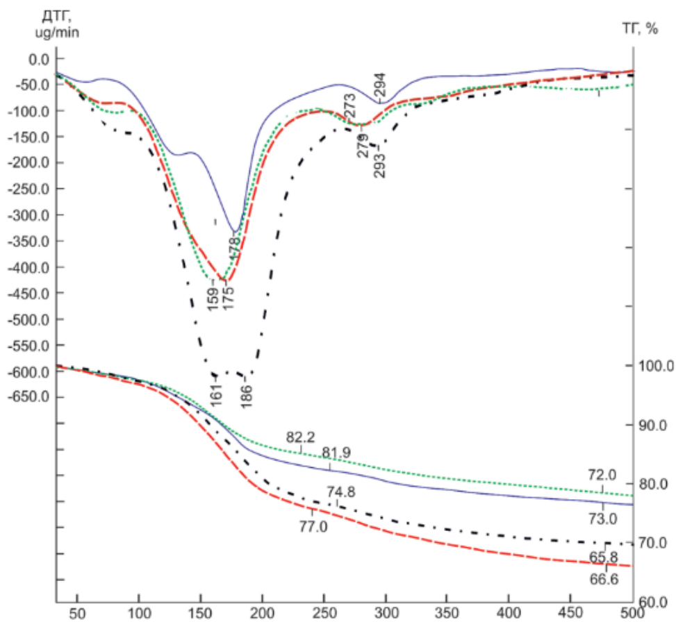
Figure 2. Curve of thermal analysis of Khaudag bentonite sample
