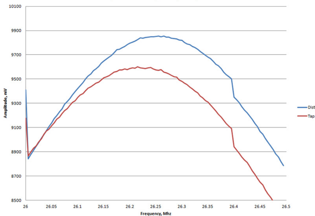
Figure 3. Amplitude-Frequency Response
